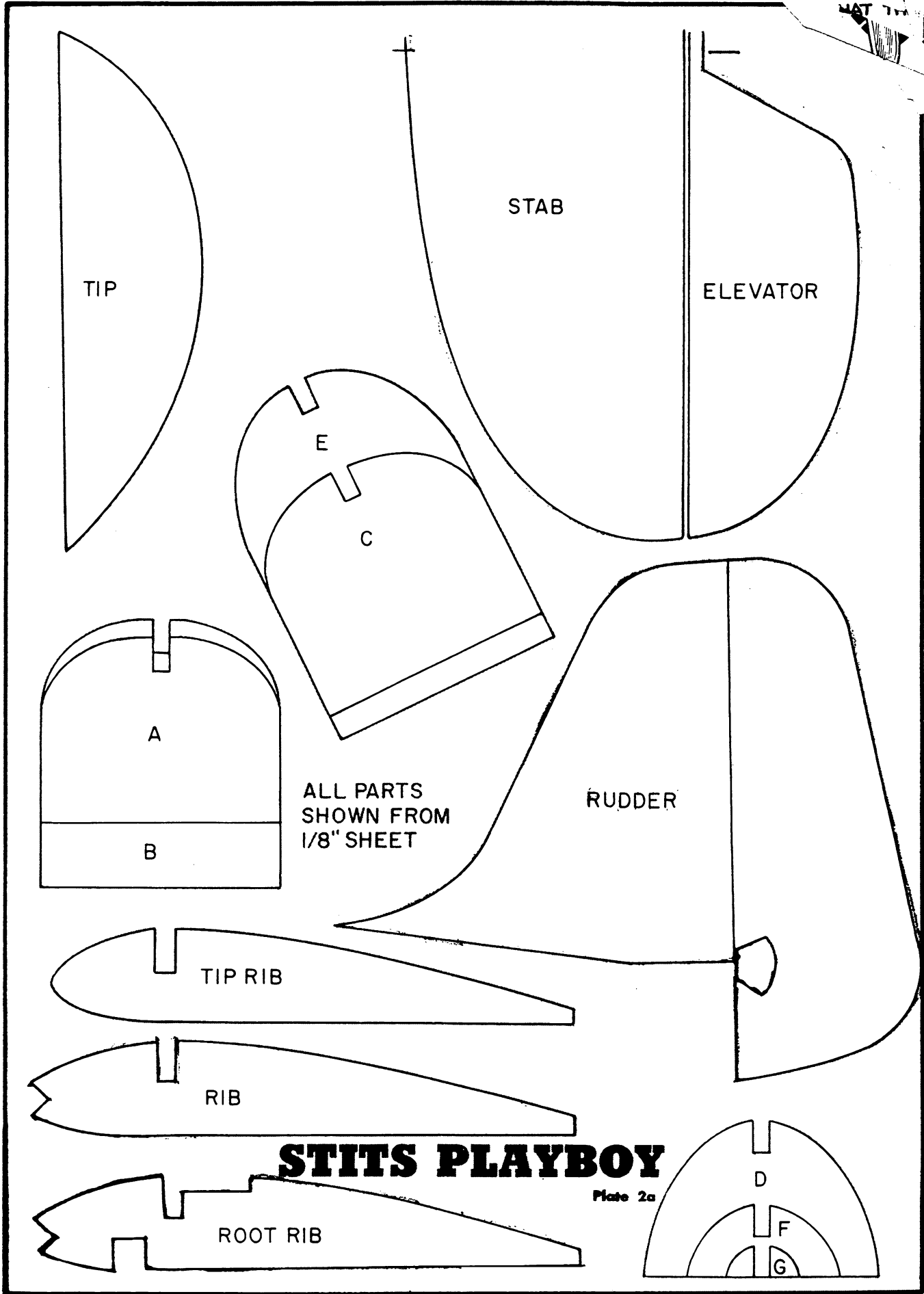
Full-Size Plan
